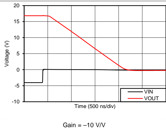
Figure 28. Positive Overload Recovery
