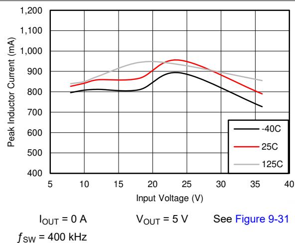
Figure 7-6. I_{PEAK-MIN}
