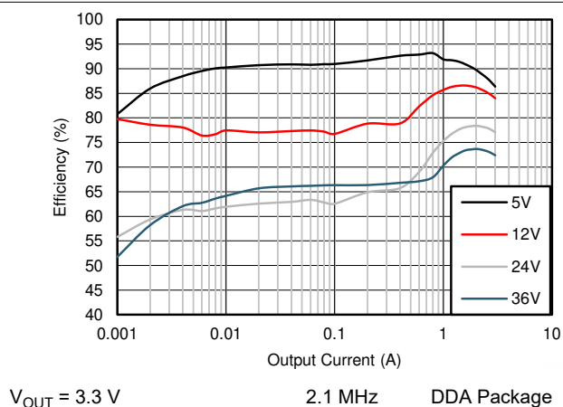
Figure 9-12. Efficiency
