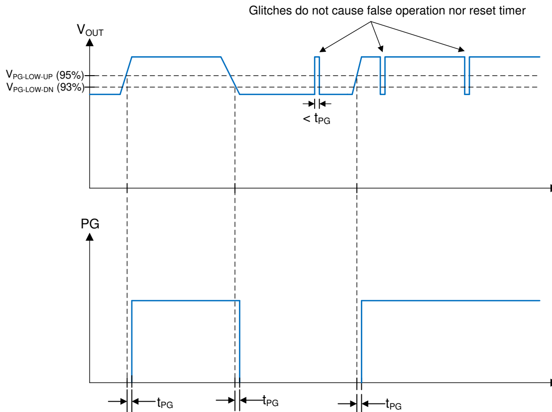
Figure 8-2. Power-Good-Timing Behavior
