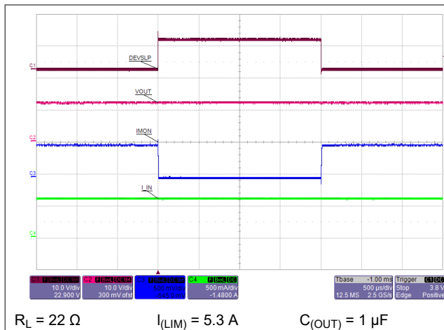
Figure 9-6. IMON Disabled in DevSleep Mode
