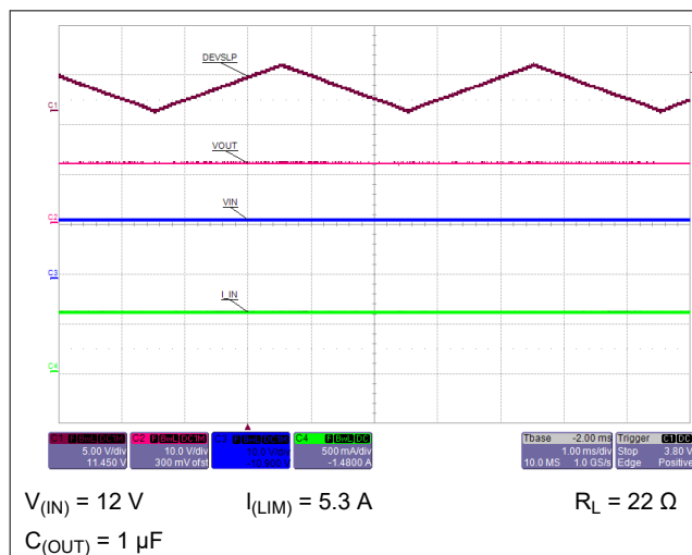
Figure 9-4. IN and OUT of DevSleep Mode with 550-mA Load
