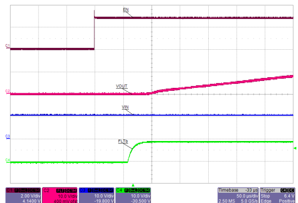
Figure 7-32. Turn ON with Enable
