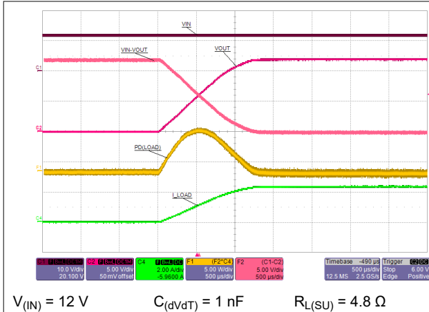
Figure 10-4. Start-Up With Load
