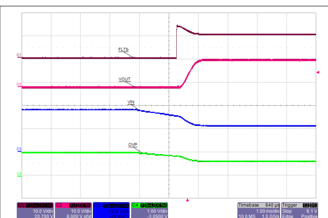
Figure 10-10. Overvoltage Recovery
