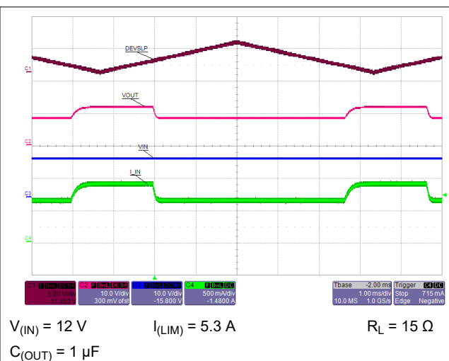
Figure 9-5. IN and OUT of DevSleep Mode with 800-mA Load. In DevSleep, Load Current Gets Limited to I_{(\text{DEVSLP}(\text{LIM}))}
