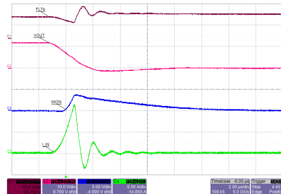
Figure 7-40. Hot-Short: Fast Trip Response and Current Regulation
