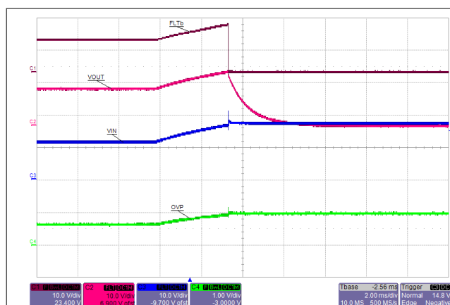
Figure 10-9. Overvoltage Shutdown
