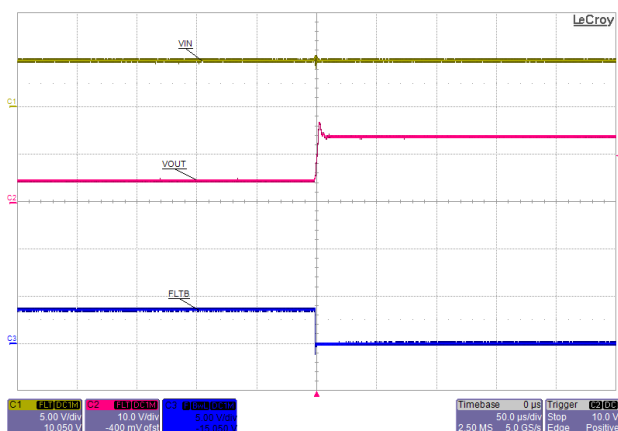
Figure 10-21. V_{BUS} Short-to-Battery Protection
