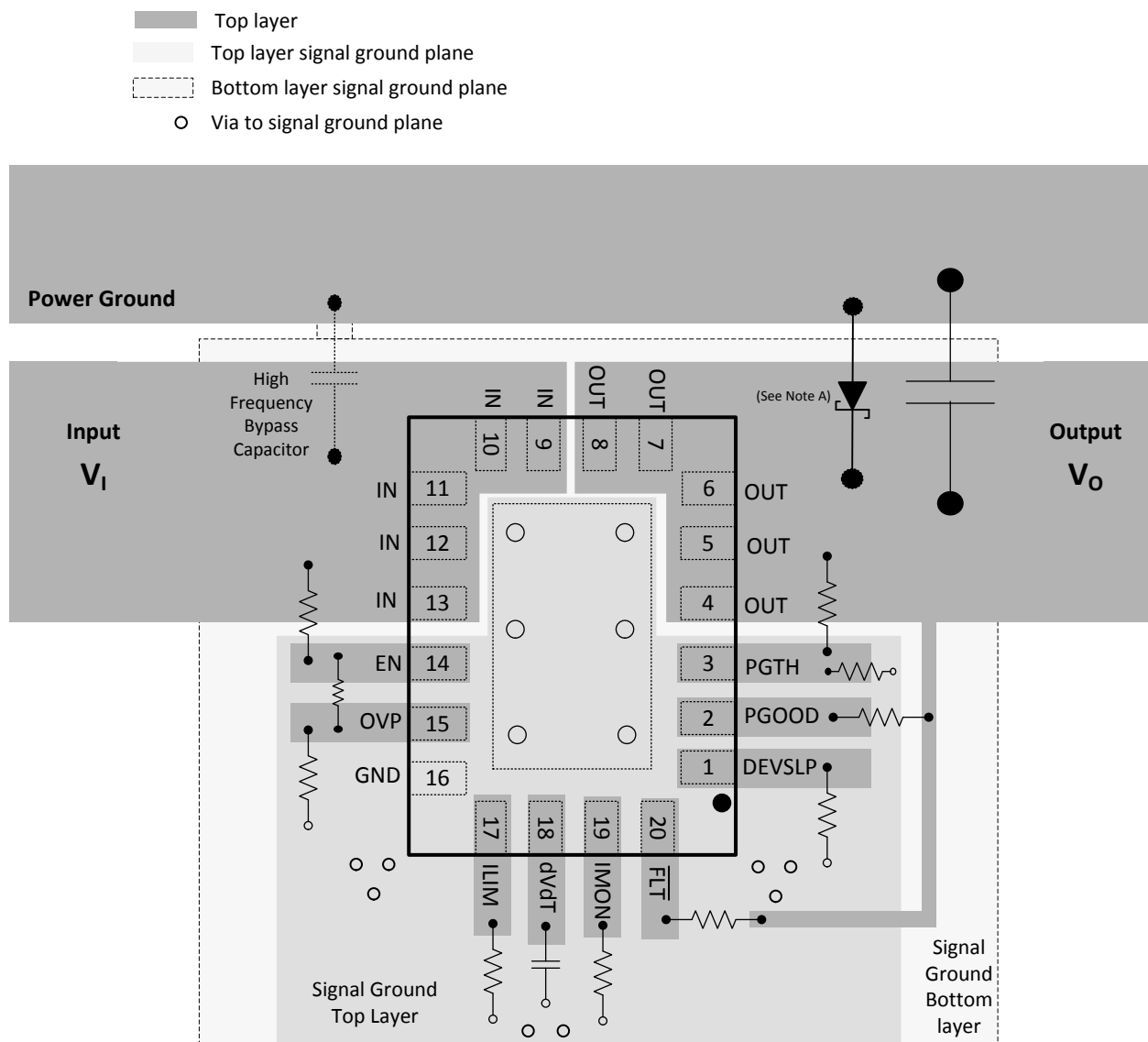
Figure 12-1. Board Layout
