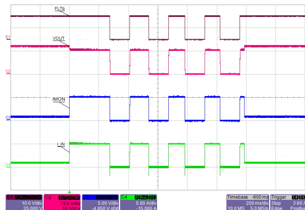
Figure 10-12. Overload Condition: Auto Retry and Recovery - TPS25940-Q1
