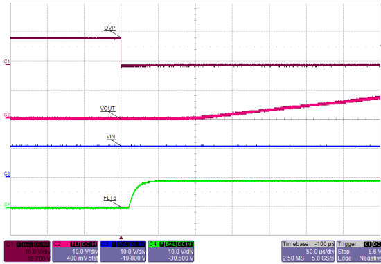
Figure 7-37. OVP Turn ON Delay: OVP \downarrow to Output Ramp \uparrow
