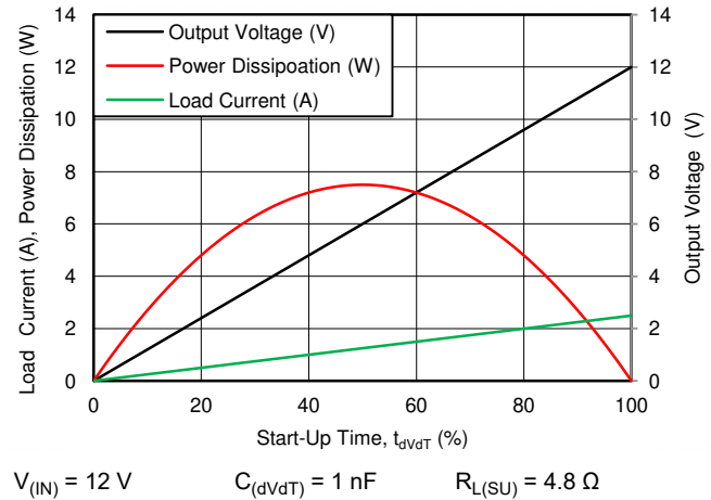
Figure 10-5. P_{D(LOAD)} in Load During Start-Up
