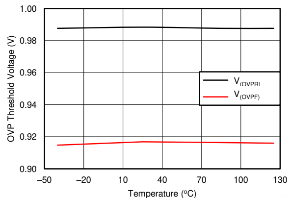
Figure 7-6. OVP Threshold Voltage vs Temperature
