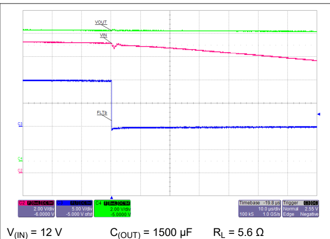
Figure 10-25. Hot-Plug Out Condition: \overline{\text{FLT}} Delay
